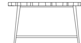
Sideboard VT40:135 h: 72 cm w: 45 cm l: 135 cm
