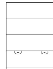
H1B* Shelves, drawer h: 147.5 cm d: 42 cm w: 90 cm
