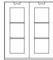
E Glass fronted cabinet h: 109 cm d: 30 cm (or 42 cm) w: 90 cm
