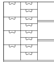
C Drawers and shelves h: 109 cm d: 42 cm w: 90 cm
